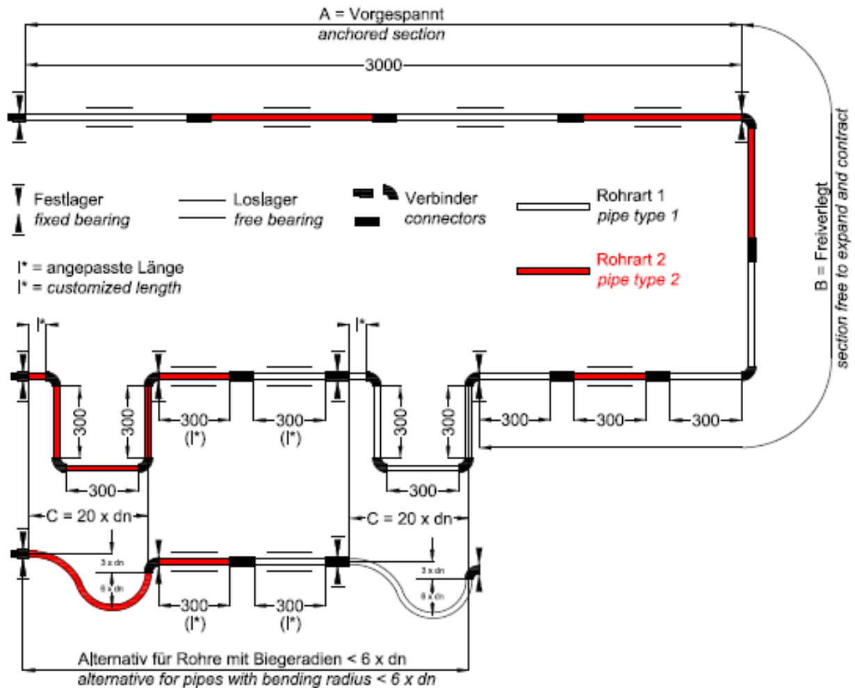
Figure 2 Temperature cycling test with one single type of connector combined with two types of pipe
